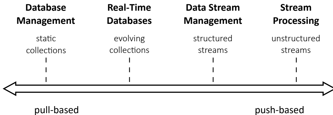
Fig. 1: Different classes of data management systems and the access patterns they support. At the one extreme, there are traditional databases which represent snapshots of domain knowledge that are the basis of all queries. At the other extreme, there are general-purpose stream processing engines which are designed to generate output from conceptually unbounded and arbitrarily structured ephemeral data streams. Real-time databases and data stream management systems both stand in the middle, but adhere to different semantics: Real-time databases work on evolving collections that are distinguished from their static counterparts (i.e. from typical database collections) through continuous integration of updates over time, enabling push-based real-time queries. Data stream management systems provide APIs to query data streams, for example, by applying filters to incoming data or by computing rolling aggregations and joins over configurable time windows.
