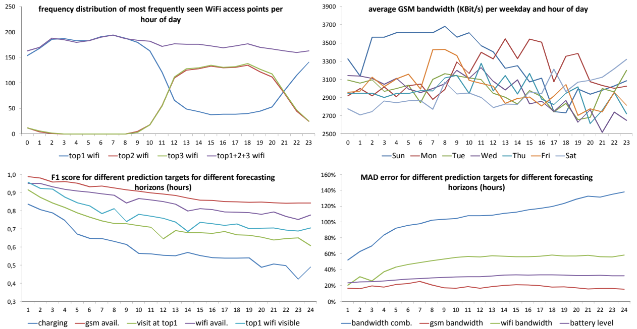
Fig. 2. Nokia MDC data characteristics (top) and evaluation of the prediction performance (bottom)
