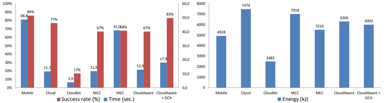
Fig. 3. CloudAware evaluation results: Consumed energy, task execution success rate and execution time
