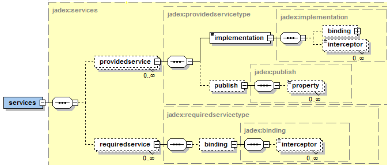
FIGURE 4.4. Provided and required service specification
