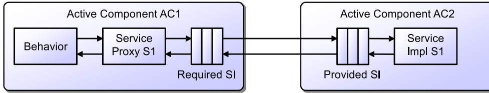
FIGURE 4.3. Service interceptors
