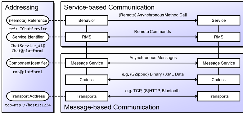
FIGURE 5.2. Jadex communication stack
