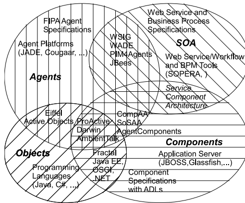
FIGURE 7.1. Paradigm integration approaches
