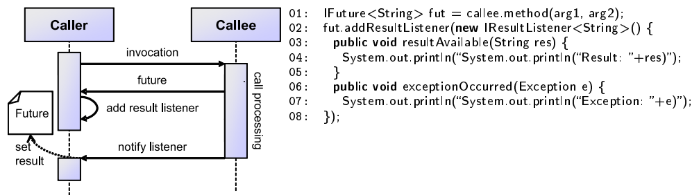
FIGURE 4.1. Asynchronous method invocation with future return value
