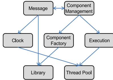
FIGURE 5.1. Basic platform services
