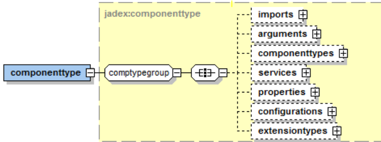
FIGURE 4.2. Active component structure specification
