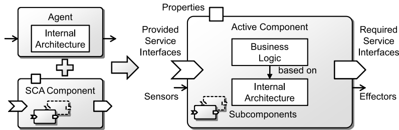
FIGURE 3.1. Active component structure
