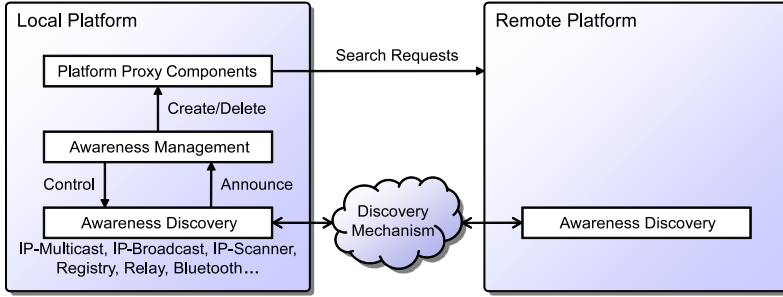
FIGURE 5.3. Jadedex platform awareness
