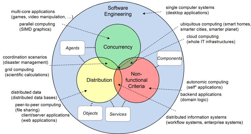
FIGURE 2.1. Applications and paradigms for distributed systems
