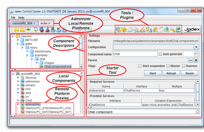
FIGURE 5.4. The Jadex control center
